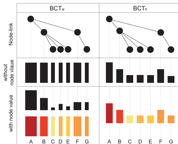
Fig. 1. BarcodeTrees (BCTs) linearize hierarchical data and map the nodes to rectangles. The BCT_w encodes the depth of each node with the Width of each rectangle, leaving height and color available for encoding node attributes. The BCT_h encodes depth with the Height of the rectangles, leaving color available for encoding node attribute values.
